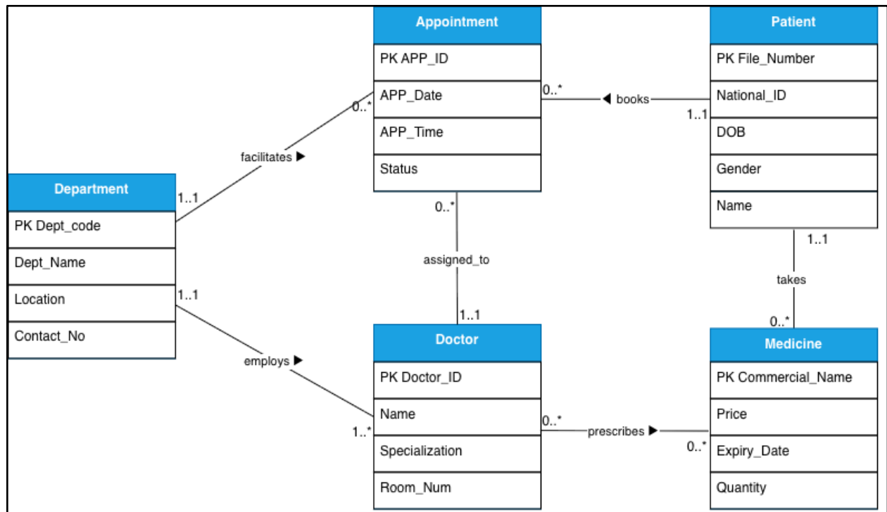
Figure 1. ERR Diagram
